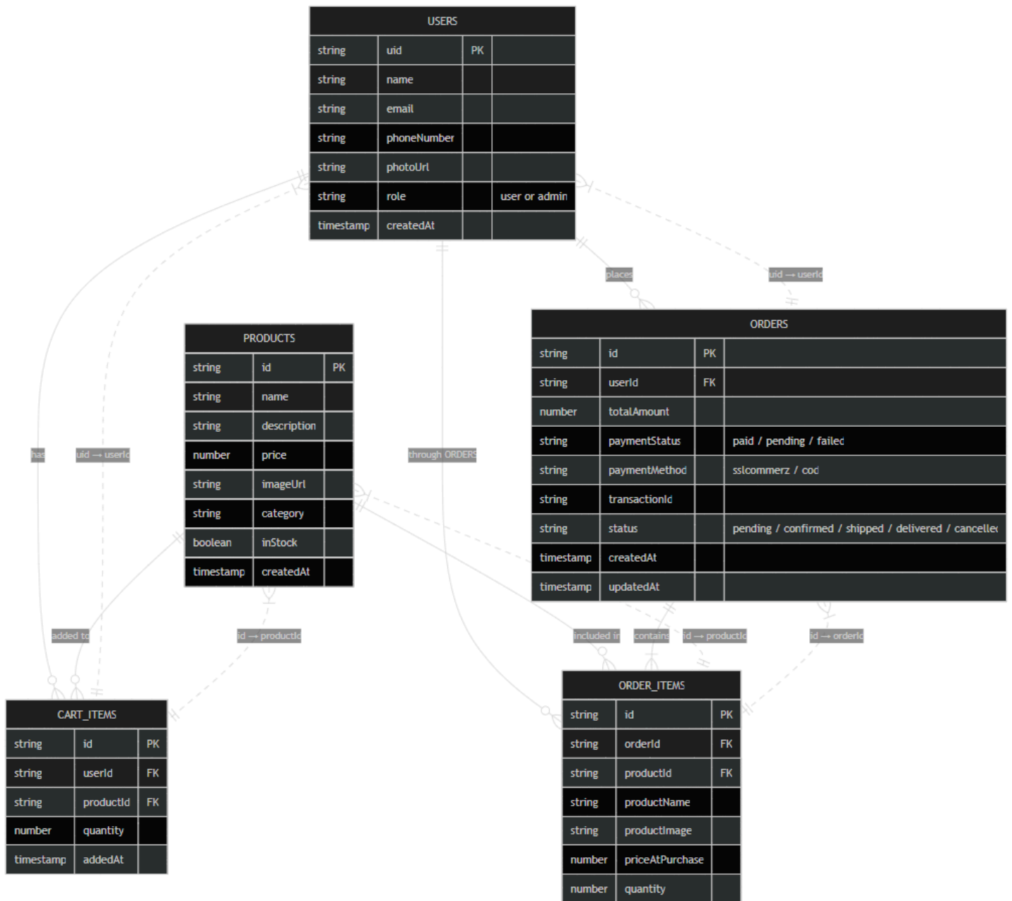
Figure 3: Entity Relationship Diagram showing relationships between Users, Products, Cart, Orders
