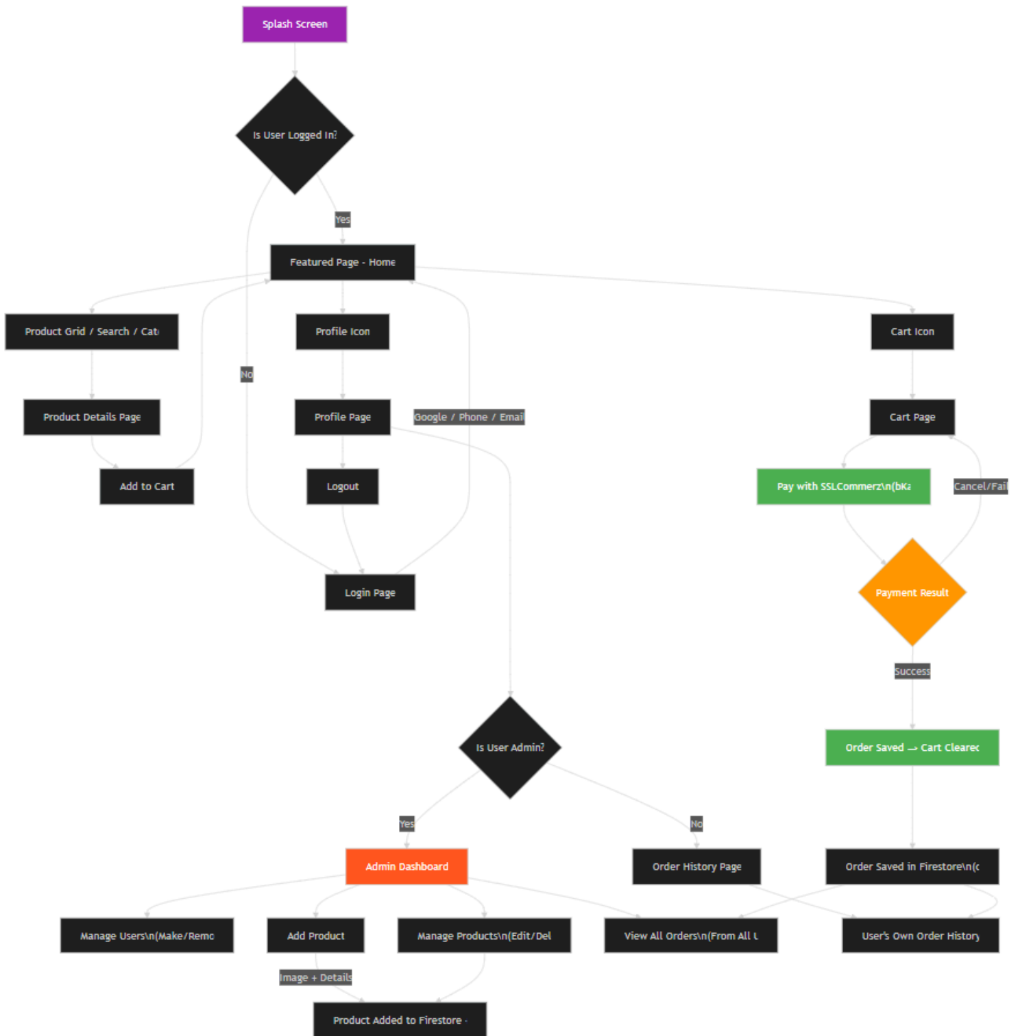
Figure 1: Complete user and admin flow of SportsShop
